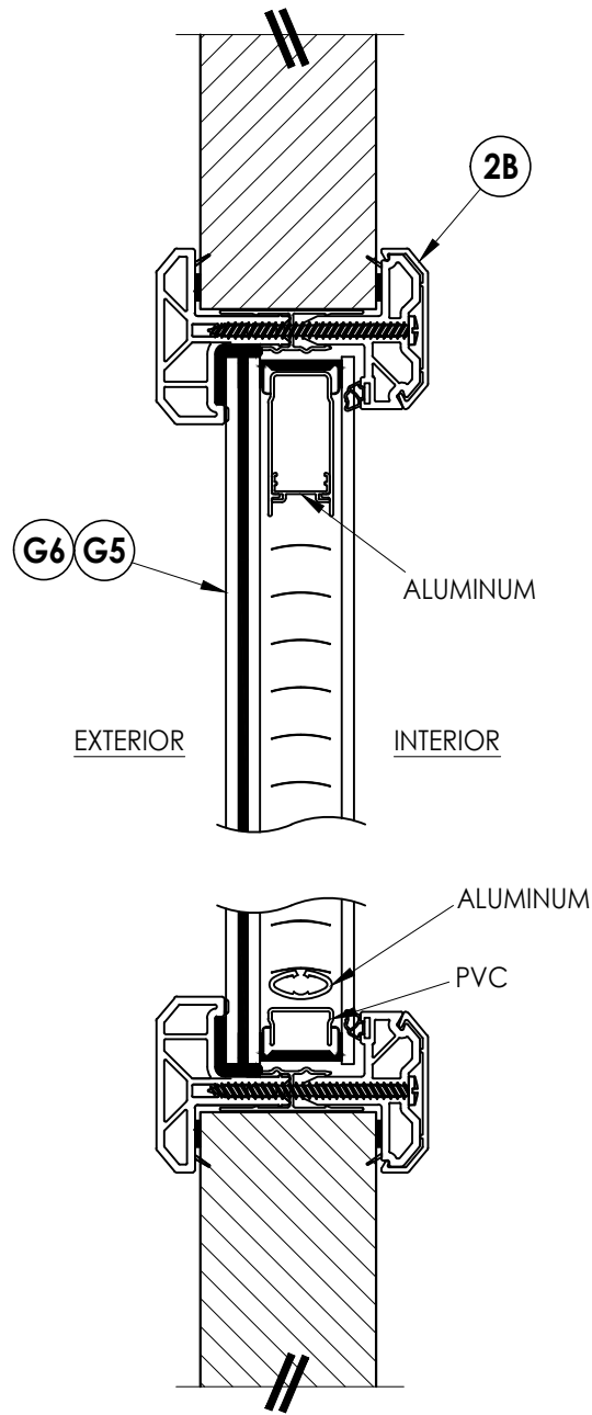
1/4 VERTICAL CROSS SECTION WARMEDGE OPERABLE BLIND
