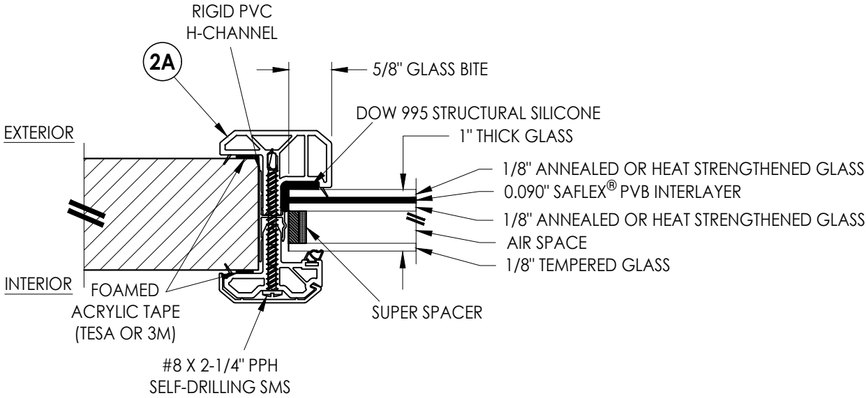
G2 GLAZING DETAIL SUPER SPACER
