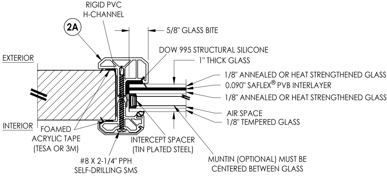
G4 GLAZING DETAIL INTERCEPT SPACER w/ OPTIONAL MUNTIN
